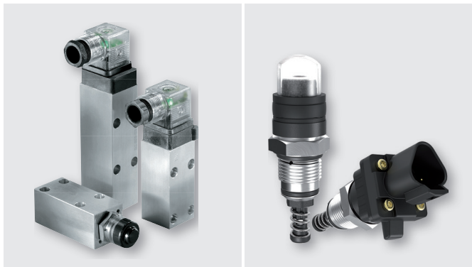
ARGO-HYTOS differential pressure indicators
