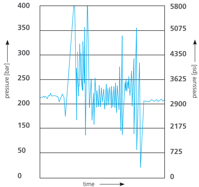
Pressure peaks
