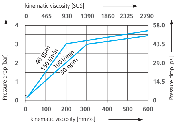
Pressure drop
