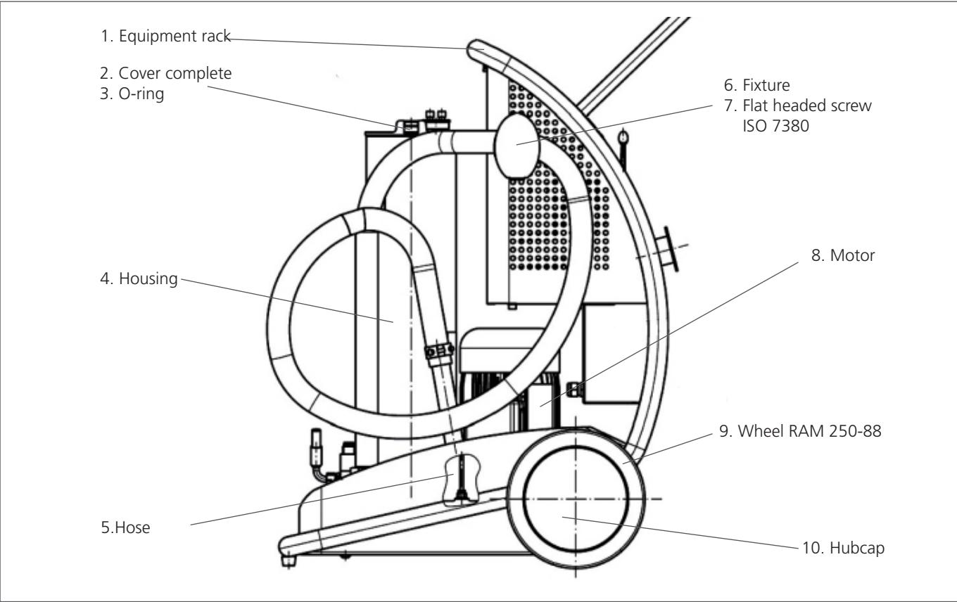
Fig. 42: Spare parts drawing 1
