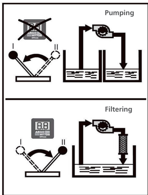
Fig. 27: Lever pumping / filtering
