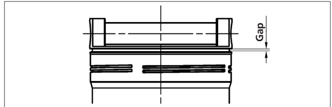
Fig. 36: Gap at the filter cover
