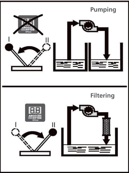
Fig. 26: Lever pumping / filtering
