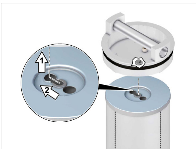
Fig. 34: Attaching the filter element
