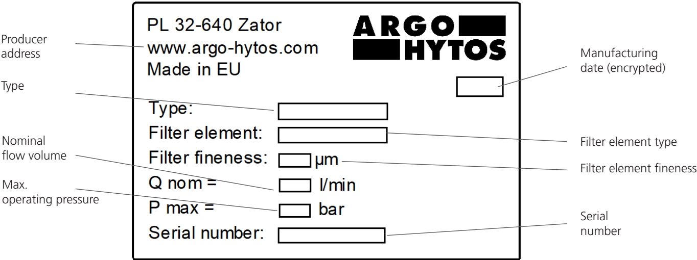
Fig.3: Nameplate
