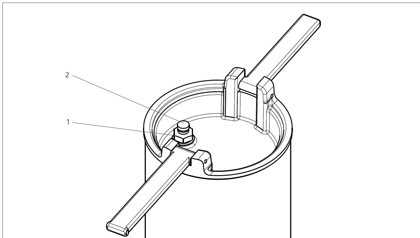
Fig.5: Venting
