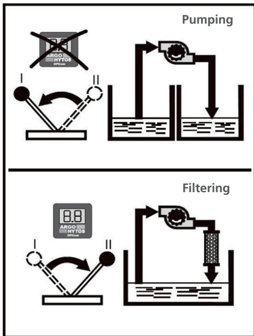
Fig. 30: Lever pumping / filtering
