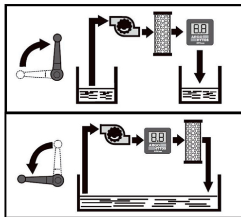
Fig. 31: Three-way valve
