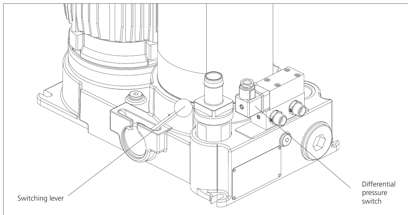
Fig.2: Component overview 2 (transport rack removed)
