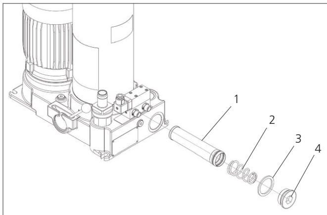
Fig. 37: Removing the suction filter
