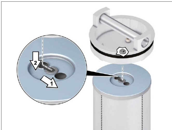
Fig. 33: Removing the filter element from the cover
