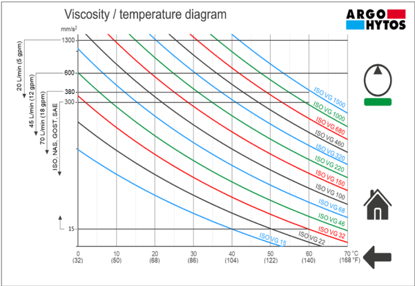
Fig. 9: Screen with viscosity / temperature diagram
