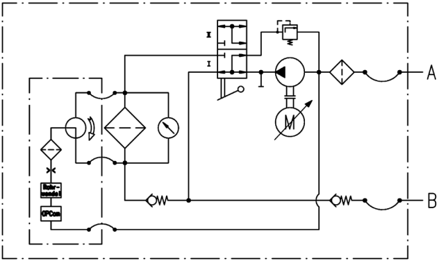
Fig. 41: Hydraulic diagram UMPC2 with variable flow
