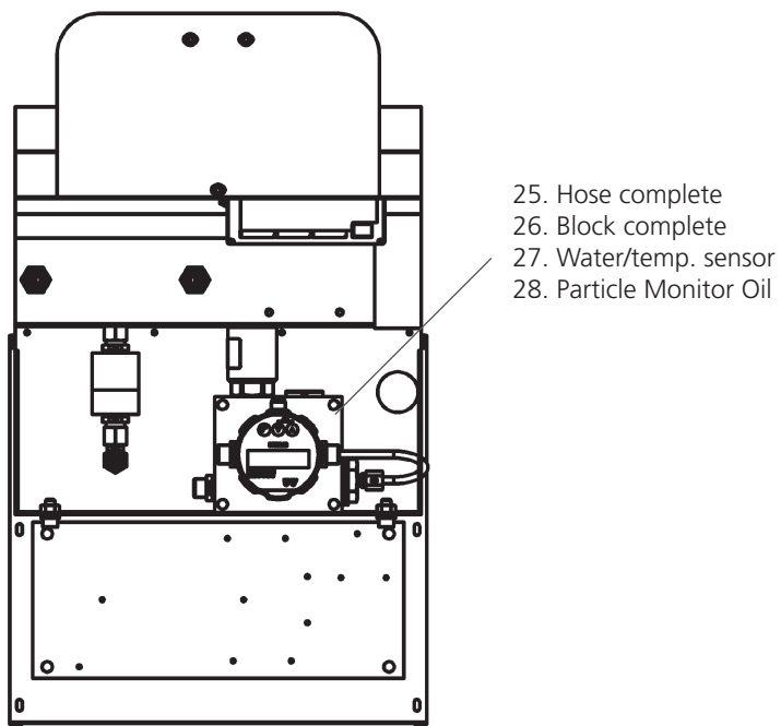
Fig. 46: Spare parts drawing 5
