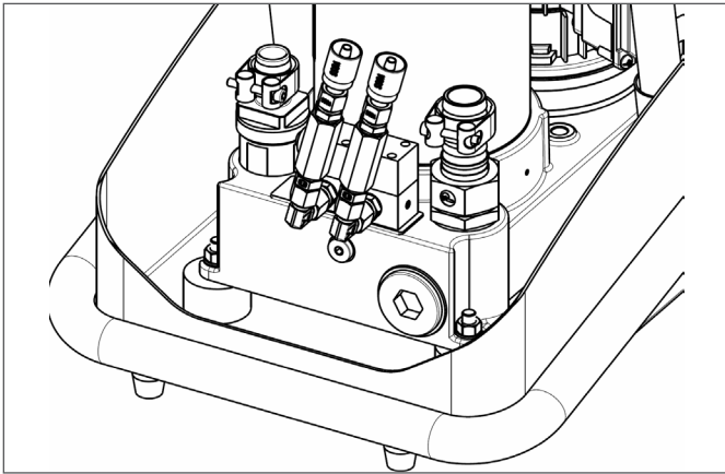
Fig. 38: Removing screen filters
