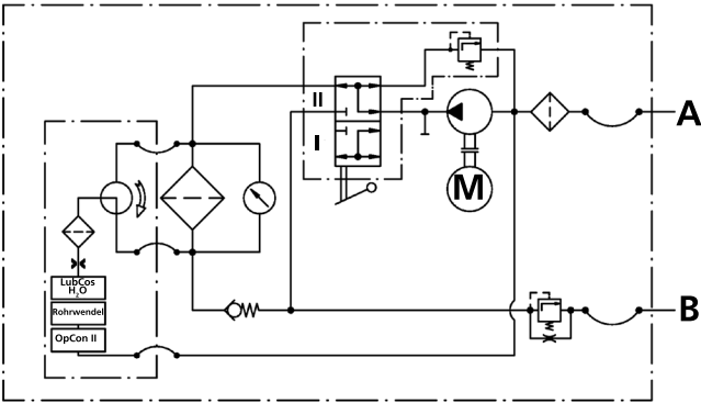
Fig. 40: Hydraulic diagram UMPC2 with fixed flow
