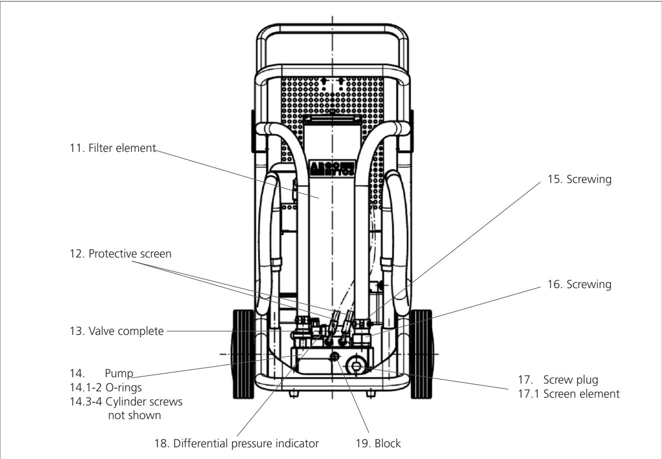
Fig. 43: Spare parts drawing 2
