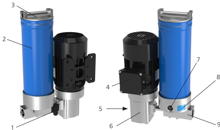
Fig. 1: Component overview
