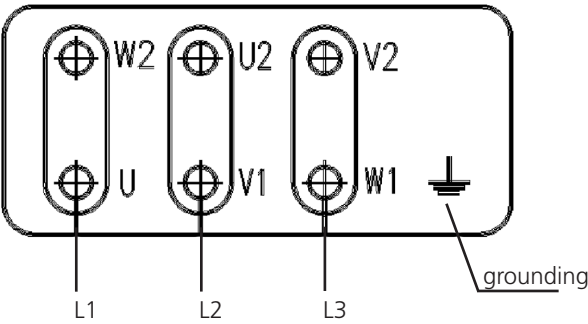
△ Delta connection
