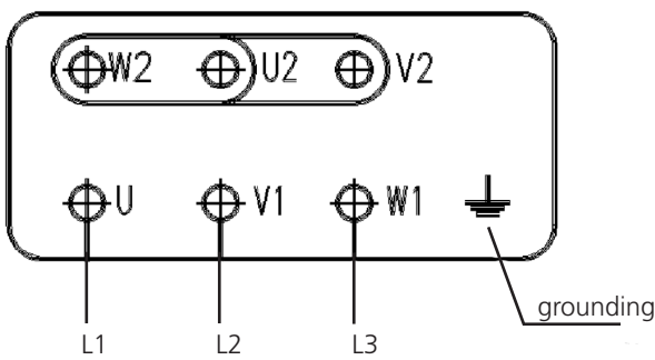
Y Star connection
