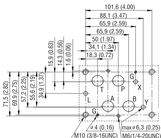
Dn 16 - ISO 4401-07-07-0-05
