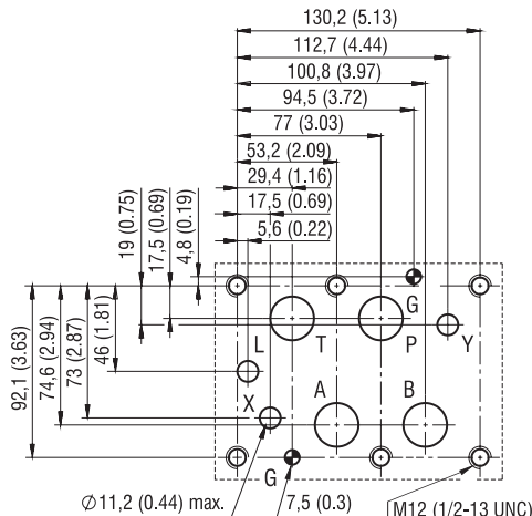
Dn 25 - ISO 4401-08-08-0-05
